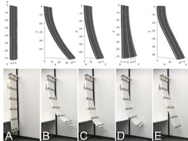
Fig. 5. Top Row: Simulation of 5 Configurations, Bottom Row: Prototype Images of Configurations.
