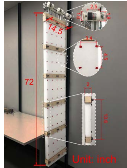
Fig. 3. Dimensions of the built prototype.
